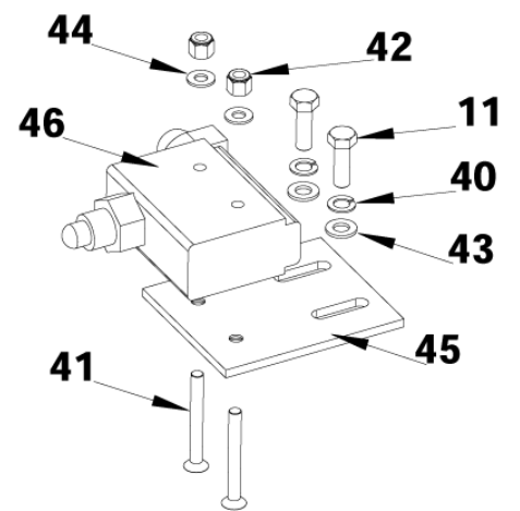
Brake pedal assembly
