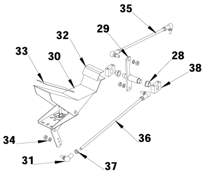
Accelerator pedal assembly
